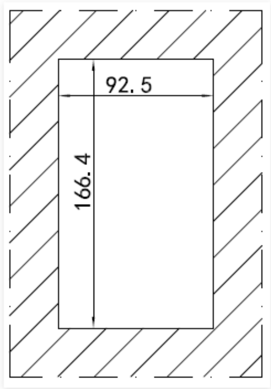
YD587 pallet cut-out size unit (mm)
